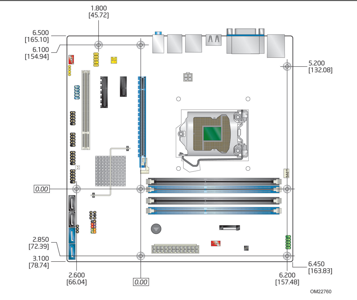
Figure 15. Board Dimensions
