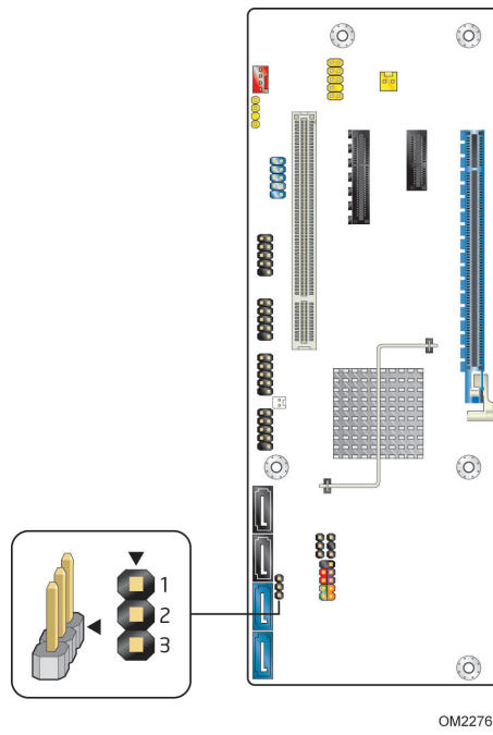
Figure 14. Intel MEBX Reset Header
